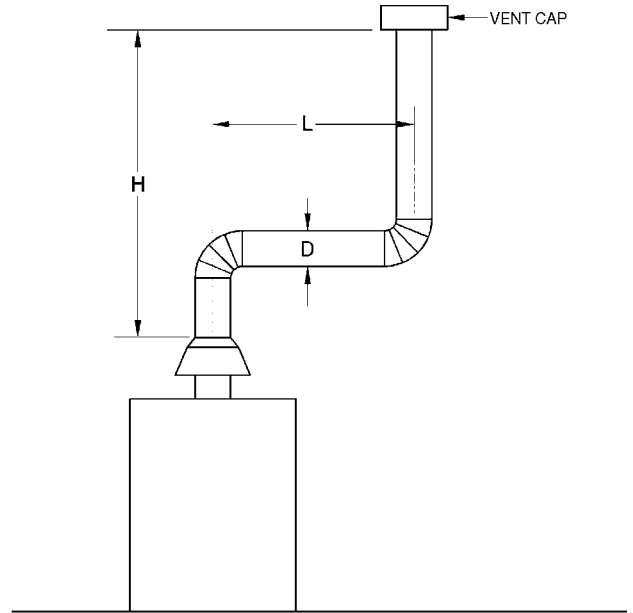
FIGURE B-5 ASBESTOS CEMENT TYPE B OR SINGLE-WALL METAL VENT SYSTEM SERVING A SINGLE DRAFT-HOOD-EQUIPPED APPLIANCE
