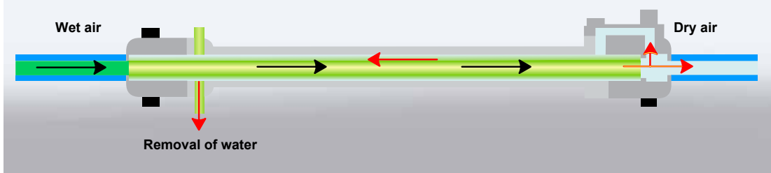
Working principle of membrane dryers.
