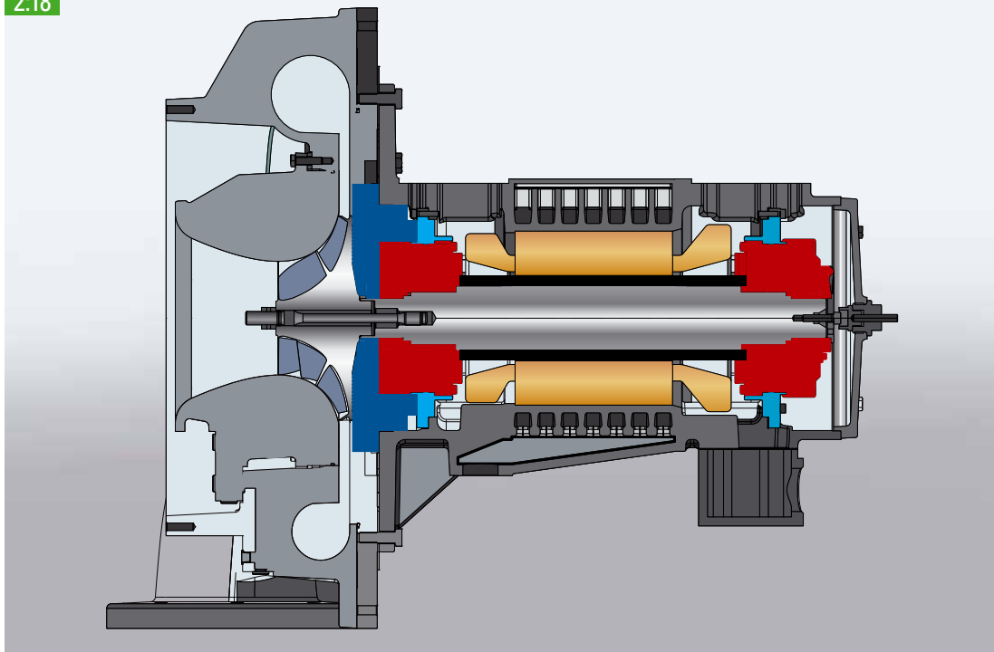
Modern high-speed direct-drive centrifugal compressor.
