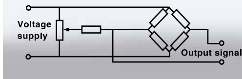
Bridge connection with strain gauges.
