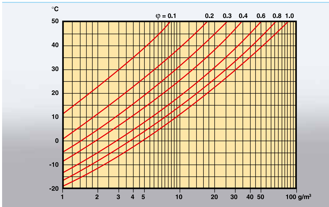
Water content in air at different relative vapor pressures (φ)
