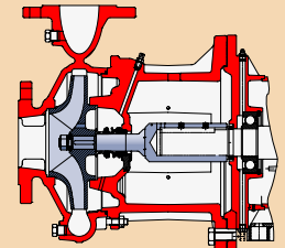
Fig. 1.1.27: Close-coupled pump with rigid coupling
