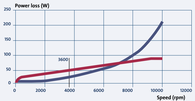
Fig. 1.3.18: Power consumption of a 12 mm mechanical shaft seal
