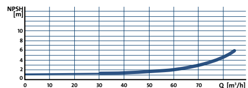
Fig. 1.1.9: The NPSH-curve of a typical centrifugal pump
