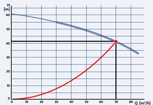
Fig. 1.1.6: A typical QH-curve for a centrifugal pump; low flow results in high head and high flow results in low head
