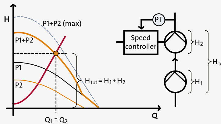
Fig. 3.2.7: Equal sized fixed speed pump and speed-controlled pump connected in series. A pressure transmitter PT together with a speed controller is making sure that the pressure is constant at the outlet of P2.
