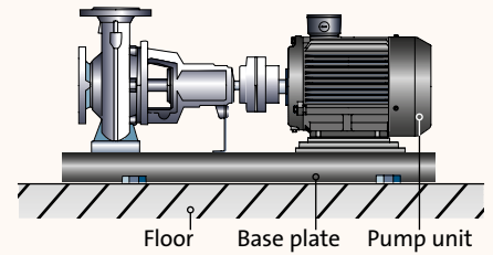
Fig. 2.1.6: Floor
